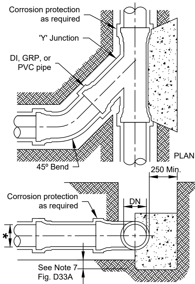
ELEVATION (FOR HORIZONTAL THRUST) THRUST BLOCK FOR 'Y's
