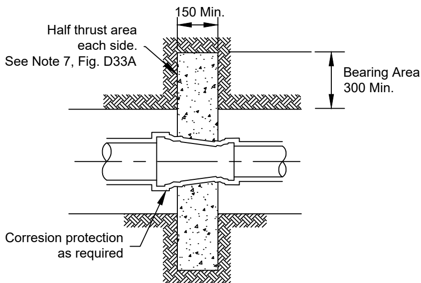
PLAN (FOR HORIZONTAL THRUST) TAPER THRUST BLOCK
