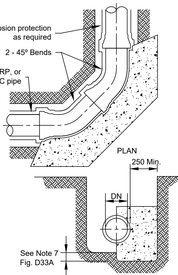
ELEVATION (FOR HORIZONTAL THRUST) THRUST BLOCK FOR BENDS
