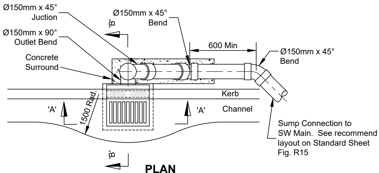
Detail of connection at back of sump
