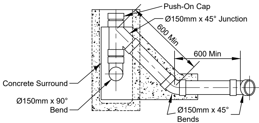
Detail of connection at back of sump
