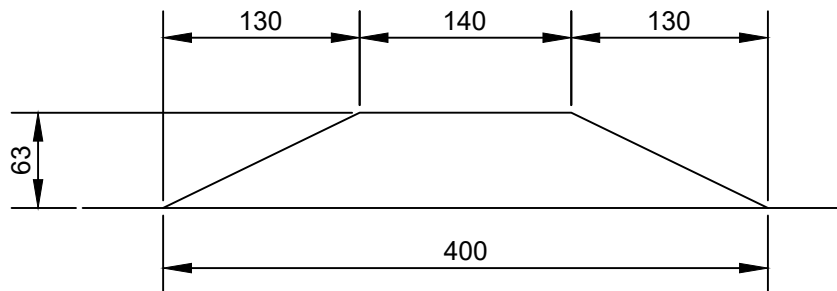
SECTION FOR SMALL PROFILE HUMPS
