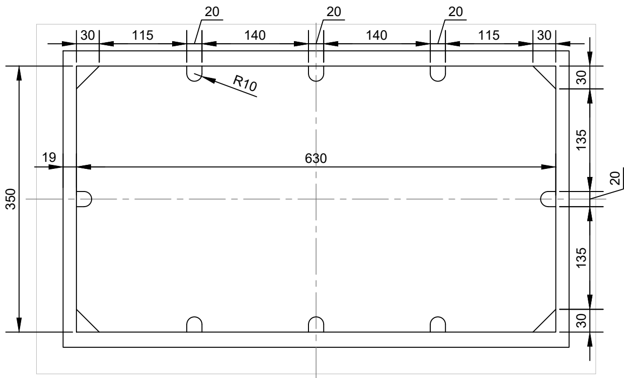
Topside
