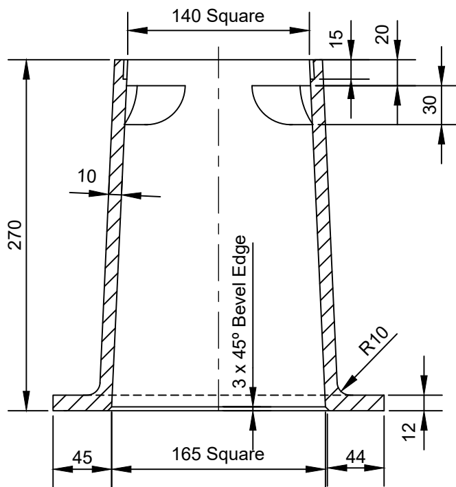
Half Section
