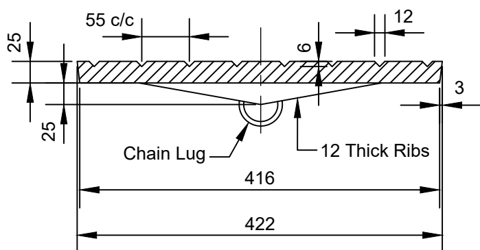
Half Section
