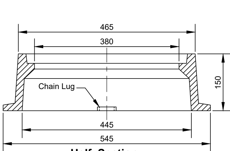
Half Section
