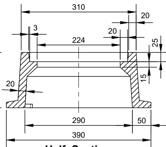
Half Section
