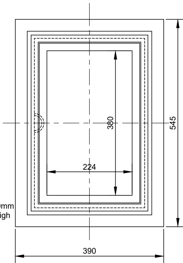
Plan of Frame
